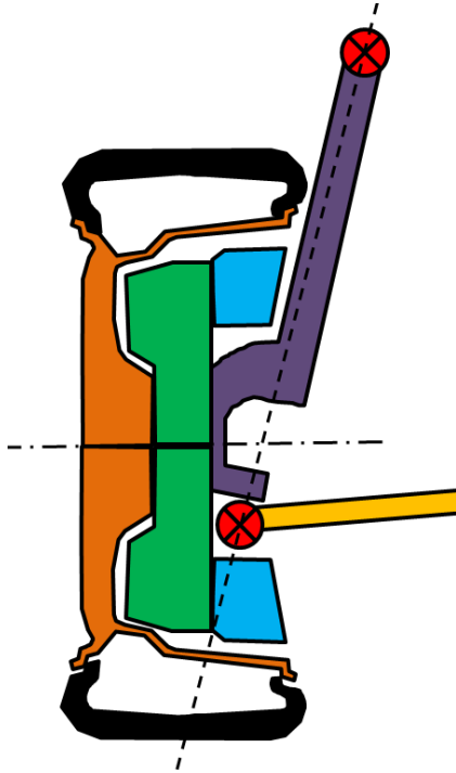
Figure 7: Toroidal volume available for rotating brake hardware in blue
